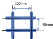
DHW51224S10050 Wire Dia. Ø5.0mm
