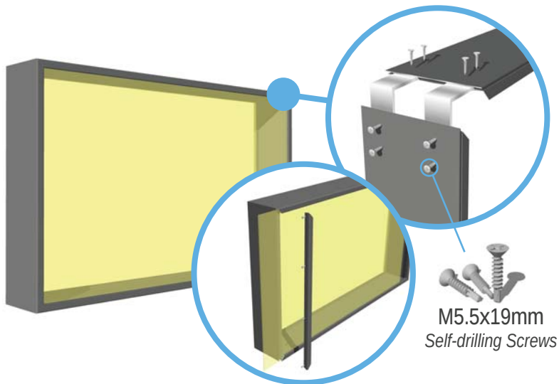
GM-NEWZ-237 Retaining Trim Profile
