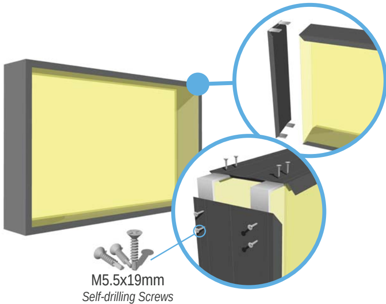
SL-455 Frame Corner Stake
