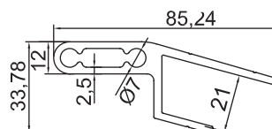
GM-NEWZ-144 GM-NEWZ-142 & 143 Holder
