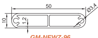
GM-NEWZ-96 50x10mm Louvre Blade 0.42kg/m
