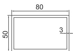
RHA80B50T3 80x50mm Louvre Blade 2.120kg/m
