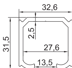
GM-NEWZ-135 Roller Sliding Track 0.72kg/m
