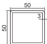
GM-NEWZ-50x50x3R 50x50mm Louvre Blade 1.67kg/m
