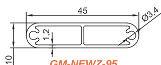
GM-NEWZ-95 45x10mm Louvre Blade 0.41kg/m
