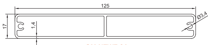
GM-NEWZ-94 125x17mm Louvre Blade 1.25kg/m
