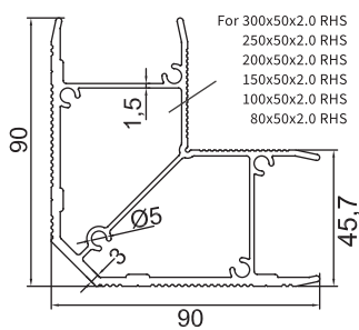
GM-NEWZ-133 50mm Corner Stake
