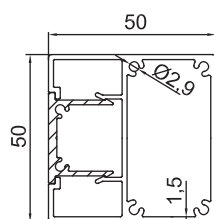
GM-NEWZ-54&53 50x50mm Louvre Blade 1.48kg/m
