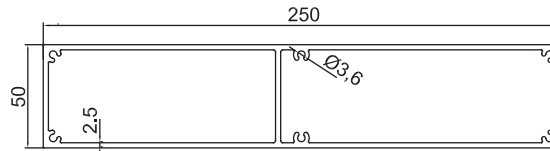
GM-NEWZ-100 250x50mm Louvre Blade 4.84kg/m
