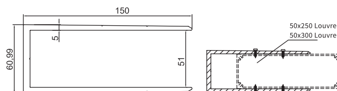
GM-NEWZ-145 50mm Louvre Blade Holder
