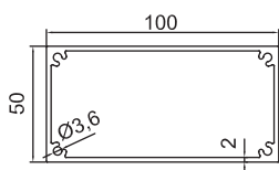
GM-NEWZ-120 100x50mm Louvre Blade 1.91kg/m
