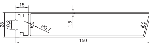
GM-NEWZ-182 150x30mm Louvre Blade 1.770kg/m
