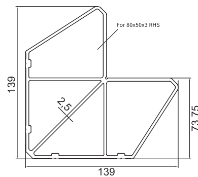
GM-KPM-123 80x50mm Corner Stake
