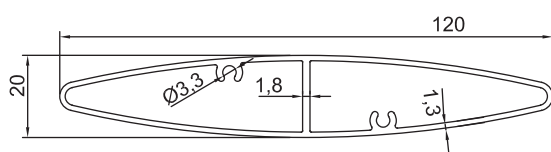
GM-NEWZ-06 120x20mm Louvre Blade 1.09kg/m
