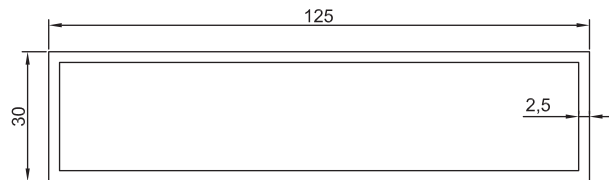
RHA125B30T2.5 125x30mm Louvre Blade 2.138kg/m
