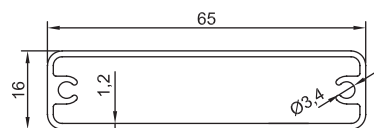
GM-NEWZ-04 65x16mm Louvre Blade 0.65kg/m
