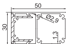
GM-NEWZ-51&53 30x50mm Louvre Blade 1.07kg/m
