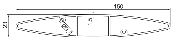
GM-NEWZ-70 150x23mm Louvre Blade 1.58kg/m
