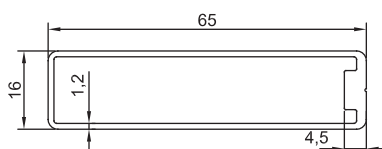
GM-NEWZ-61 65x16mm Louvre Blade 0.69kg/m
