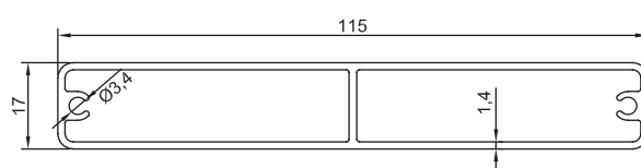
GM-NEWZ-93 115x17mm Louvre Blade 1.16kg/m
