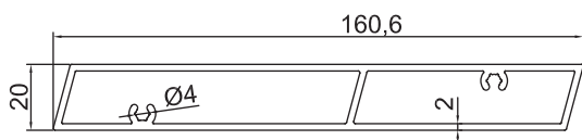
GM-NEWZ-143 160.6x20mm Louvre Blade 2.21kg/m
