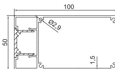
GM-NEWZ-55&53 50x100mm Louvre Blade 1.91kg/m
