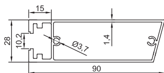
GM-NEWZ-181 100x30mm Louvre Blade 1.210kg/m
