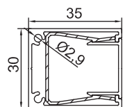
GM-NEWZ-56&57&58 30x35mm Louvre Blade 0.77kg/m
