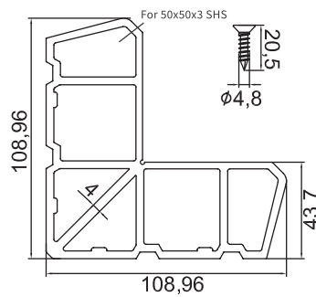
GM-KPM-5511 50x50mm Corner Stake
