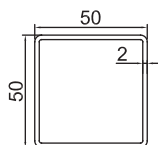
GM-NEWZ-50x50x2R 50x50mm Louvre Blade 1.13kg/m
