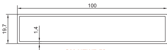
GM-NEWZ-59 100x19.7mm Louvre Blade 0.88kg/m
