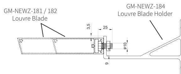
GM-NEWZ-184 Louvre Blade Holder 4.690kg/m
