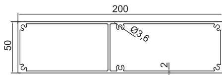
GM-NEWZ-101 200x50mm Louvre Blade 3.46kg/m
