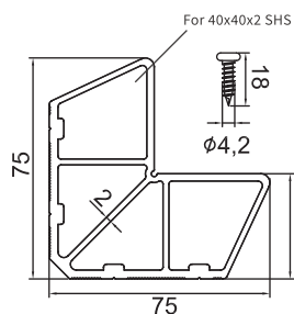
GM-NEWZ-122 40x40mm Corner Stake
