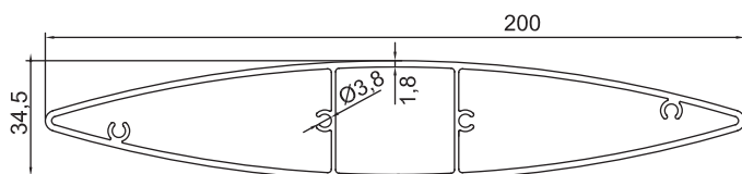
GM-NEWZ-102 200x34.5mm Louvre Blade 2.45kg/m
