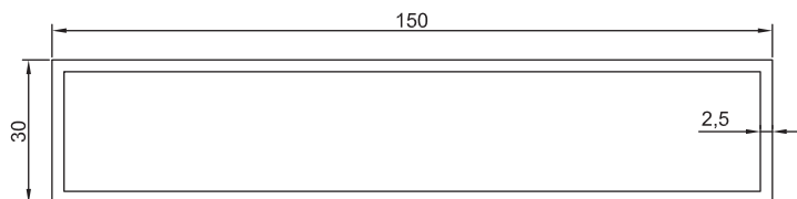
RHA150B30T2.5 150x30mm Louvre Blade 2.494kg/m
