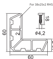
GM-NEWZ-121 38x25mm Corner Stake
