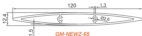
GM-NEWZ-65 120x12.4mm Louvre Blade 1.17kg/m
