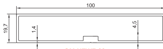
GM-NEWZ-60 100x19.7mm Louvre Blade 0.93kg/m
