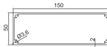
GM-NEWZ-98 150x50mm Louvre Blade 2.48kg/m
