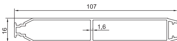
GM-NEWZ-05 107x16mm Interlock Louvre Blade 0.94kg/m
