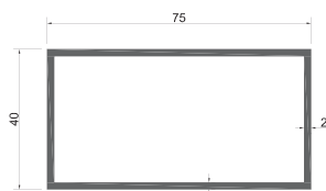
GM-NEWZ-75x40x2 GM-NEWZ-06 Hole Weight: 1.265kg/m
