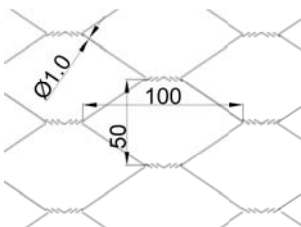
50mm Residential Mesh Aperture Detail
