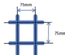
DHW531224S75 Wire Dia. Ø5.3mm
