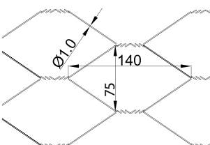
75mm Residential Mesh Aperture Detail
