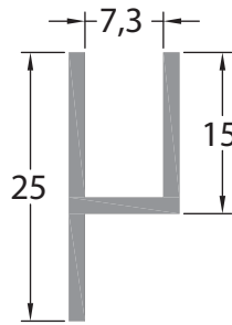
GM-NEWZ-151 Security Mesh Frame 0.217 kg/m
