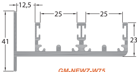
GM-NEWZ-W75 Wide Double Sliding Track 1.560 kg/m
