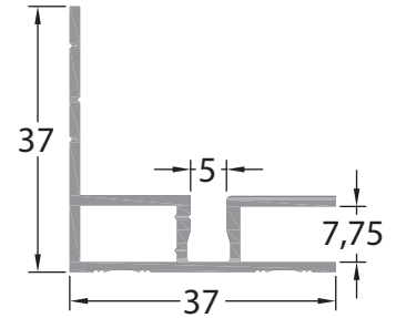
GM-NEWZ-W35 Stand-out Window Frame 0.474 kg/m
