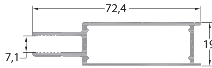
GM-NEWZ-W26 Security Door Wide Frame 0.718 kg/m
