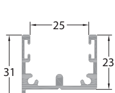
GM-NEWZ-W30 Top Sliding Track 0.510 kg/m
