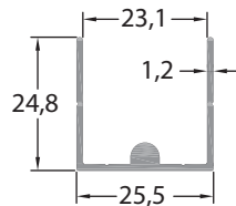
GM-NEWZ-W74 Single Sliding Track 0.300 kg/m
