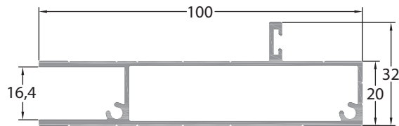
GM-NEWZ-W28 Security Door Wide Stand-out Frame 1.100 kg/m
