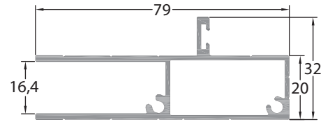
GM-NEWZ-W24 Security Door Stand-out Frame 1.000 kg/m
