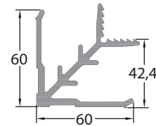
GM-NEWZ-W27 Corner Stake
