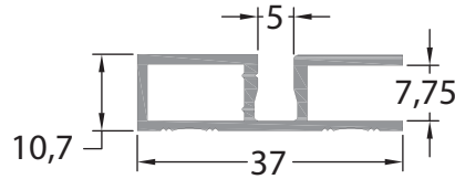
GM-NEWZ-W34 Security Window Frame 0.370 kg/m
