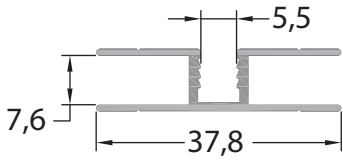
GM-NEWZ-W33 Security Mesh Jointer 0.273 kg/m
