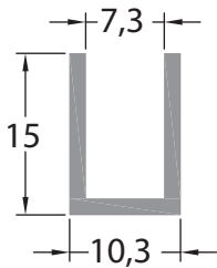
CLSA0.3B5T1.5 Security Mesh Frame 0.154 kg/m
