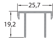
GM-NEWZ-W76 Sliding Track Top Cap 0.268 kg/m
