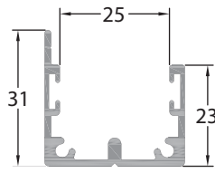
GM-NEWZ-W32 Bottom Sliding Track 0.510 kg/m
