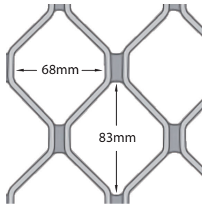
Diamond Size: 68 x 83 mm Grille Thickness: 7.0 mm
