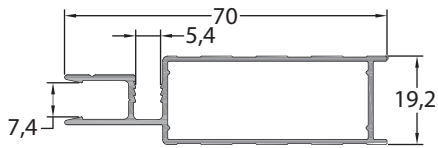
GM-NEWZ-W25 Security Door Frame 0.528 kg/m
