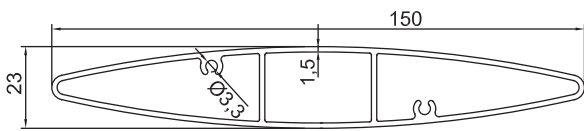
GM-NEWZ-70 150x23mm Louvre Blade 1.58kg/m
