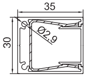
GM-NEWZ-56&57&58 30x35mm Louvre Blade 0.77kg/m
