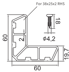
GM-NEWZ-121 38x25mm Corner Stake
