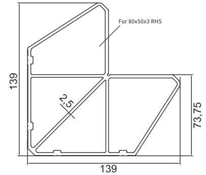
GM-KPM-123 80x50mm Corner Stake
