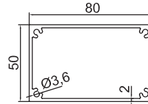
GM-NEWZ-97 80x50mm Louvre Blade 1.68kg/m
