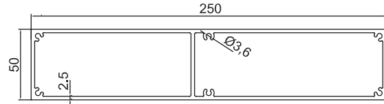
GM-NEWZ-100 250x50mm Louvre Blade 4.84kg/m
