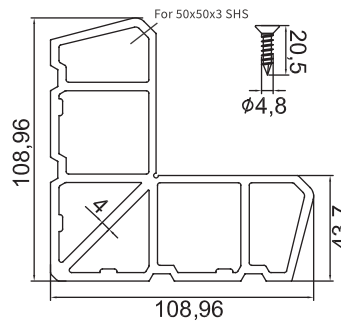
GM-KPM-5511 50x50mm Corner Stake
