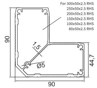
GM-NEWZ-134 50mm Corner Stake
