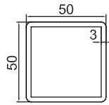
GM-NEWZ-50x50x3R 50x50mm Louvre Blade 1.67kg/m
