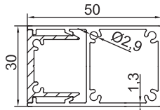
GM-NEWZ-51&53 30x50mm Louvre Blade 1.07kg/m
