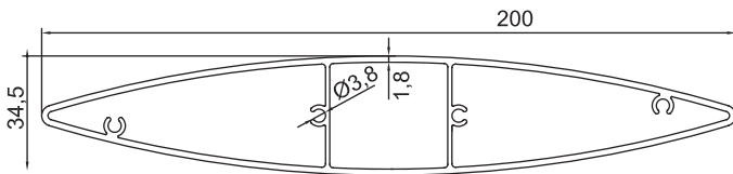
GM-NEWZ-102 200x34.5mm Louvre Blade 2.45kg/m
