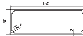
GM-NEWZ-98 150x50mm Louvre Blade 2.48kg/m
