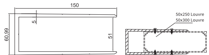
GM-NEWZ-145 50mm Louvre Blade Holder
