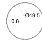
RTD49.5T0.8 Universal - Ø49.5mm Drain Pipe
