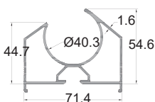
GM-NEWZ-Y13069 Universal - Top Beam Pivot Slot
