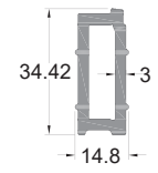
GM-NEWZ-Y13022 A3 - Frame Extend Pillar
