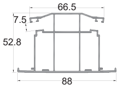
GM-NEWZ-Y13005 A3 - Premium Frame
