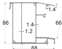
GM-NEWZ-Y13071 A5 - Wall Edge with Slot
