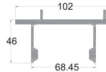
GM-NEWZ-Y13040 A8 - Bottom Joinder for 100mm
