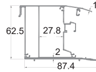
GM-NEWZ-Y13072 A3 - Wall Edge with Slot
