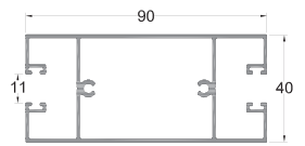
GM-NEWZ-W65 Hinge Door Middle Stile
