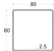
GM-80x80x2.5R A5 - 80mm Post
