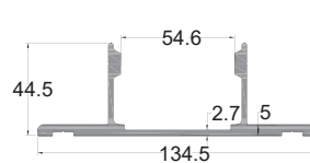
GM-NEWZ-Y13004 A3 - Bottom Jointer (Style #1)
