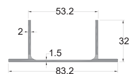
GM-NEWZ-Y13025 A3 - Bottom Jointer (Style #2)
