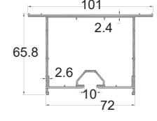
GM-NEWZ-Y13003 A3 - Flat Top Beam
