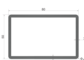
WZ-80x50x3R 25.8mm Square Hole Weight: 2.100kg/m
