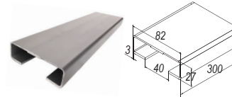
SL-280 - FG01A Aluminium Sliding Guide Weight: 0.3kg
