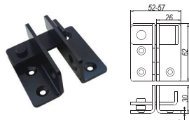
SL-271 - JCX53R Safety Gate Latch - Right Side Open Material: Galvanised Steel Weight: 0.2kg
