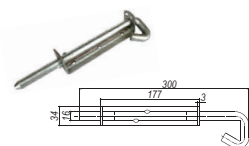
SL-293 - CX25A 300mm Drop Bolt Material: Galvanised Steel Weight: 0.8kg
