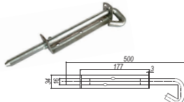
SL-294 - CX25B 500mm Drop Bolt Material: Galvanised Steel Weight: 1.1kg
