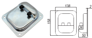
SL-267 - MX02B Swing Gate Stopper with Rubber Material: Galvanised Steel Weight: 0.5kg
