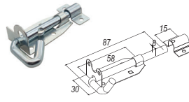
SL-291 - CX26A 87mm Sliding Pad Bolt Material: Galvanised Steel Colour Options: Galvanised Finished / Matt Black Weight: 75g
