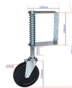
SL-282 - ZCL5"-A 5" Swivel Gate Castor Over Height: 350mm Wheel Dia.: Ø123mm
