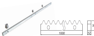
SL-284 - CT01E Sliding Gate Steel Gear Rack Length: 1000mm Fixing Hole: M4 Weight: 2.6kg
