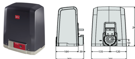
BFT DEIMOS BT-A400 Automation Sliding Gate Motor Motor Voltage: 24V Max Gate Weight: 400kg Gate Speed: 12 m/min Locking: Mechanical
