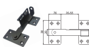
SL-271 - JCX54A Gate Flip Latch Material: Galvanised Steel Weight: 0.2kg
