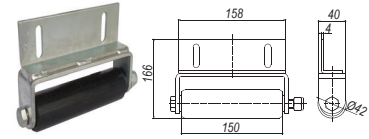
SL-278 - KJ13A.02 Adjustable Roller Guide with Bracket Material: Galvanised Steel Weight: 1.5kg
