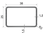
GM-NEWZ-38x25x1.5R Ø20mm Round Hole Weight: 0.523kg/m
