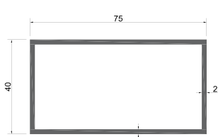
GM-NEWZ-75x40x2 GM-NEWZ-06 Hole Weight: 1.265kg/m
