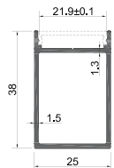
GM-NEWZ-68 20mm Square Hole Weight: 0.50kg/m
