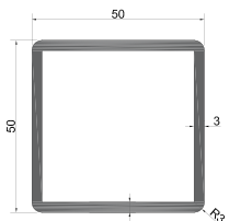
GM-NEWZ-50x50x3R Ø20mm Round Hole Weight: 1.67kg/m
