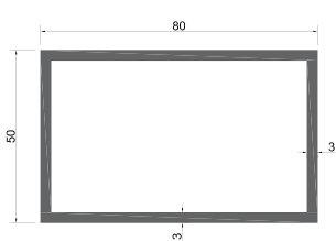
GM-NEWZ-80x50x3 GM-NEWZ-06 Hole Weight: 2.33kg/m
