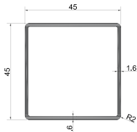
GM-NEWZ-45x45x1.6R 25.6mm Square Hole Weight: 0.783kg/m
