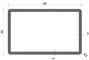
WZ-80x50x3R 25.8mm Square Hole Weight: 2.100kg/m
