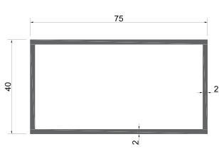
GM-NEWZ-75x40x2 GM-NEWZ-06 Hole Weight: 1.265kg/m
