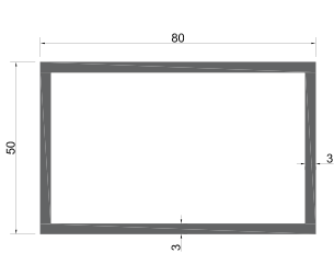
GM-NEWZ-80x50x3 GM-NEWZ-06 Hole Weight: 2.12kg/m
