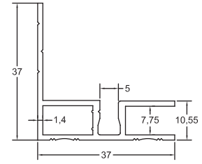
GM-NEWZ-W35 Long Leg Window Frame 0.474 kg/m
