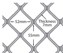
Aluminium 52x55 Grille
