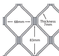
Aluminium 68x83 Grille
