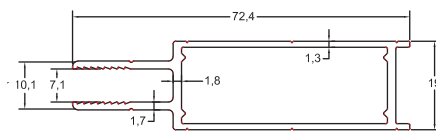
GM-NEWZ-W26 Wide Frame 0.718 kg/m
