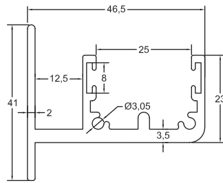
GM-NEWZ-W31 Wide Track 0.984 kg/m
