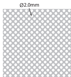
Hole Size: Ø2.00 mm Screen Thickness: 1.60 mm
