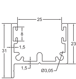
GM-NEWZ-W30 Top Track 0.510 kg/m
