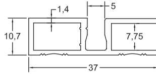
GM-NEWZ-W33 Window Frame 0.370 kg/m
