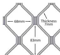
Aluminium 68x83 Grille
