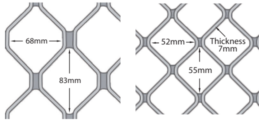
Diamond Size: 68 x 83 mm Grille Thickness: 7.0 mm
