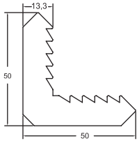
GM-NEWZ-W36 Corner Stake 1.100 kg/m
