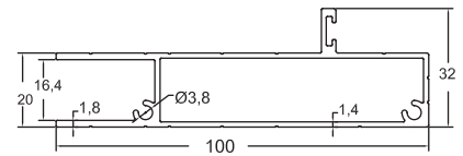
GM-NEWZ-W28 Wide Standout Frame 1.100 kg/m
