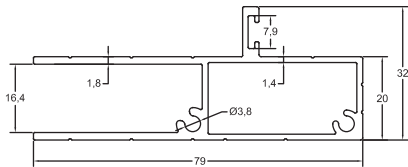
GM-NEWZ-W24 Standout Frame 1.000 kg/m
