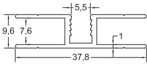
GM-NEWZ-W33 Mesh Jointer 0.273 kg/m
