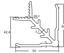
GM-NEWZ-W27 Corner Stake 2.300 kg/m
