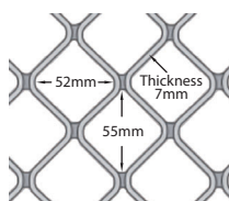
Aluminium 52x55 Grille
