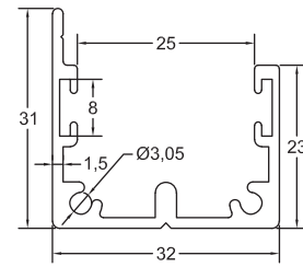
GM-NEWZ-W32 Bottom Track 0.510 kg/m
