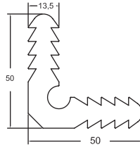
GM-NEWZ-W37 Corner Stake 1.160 kg/m
