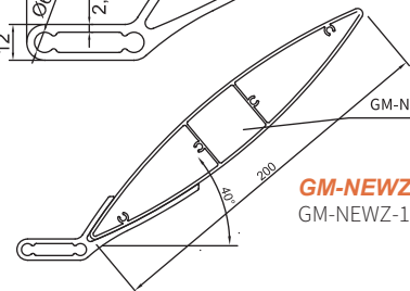
GM-NEWZ-102 200x34.5mm Louvre Blade 2.45kg/m
