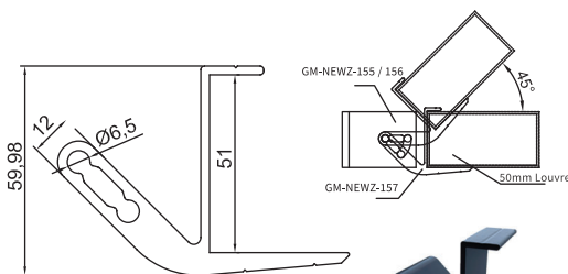
GM-NEWZ-157 50mm Louvre Blade Holder
