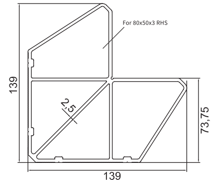
GM-KPM-123 80x50mm Corner Stake
