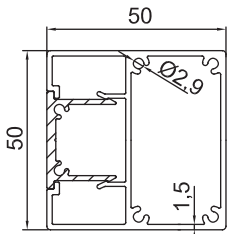
GM-NEWZ-54&53 50x50mm Louvre Blade 1.48kg/m
