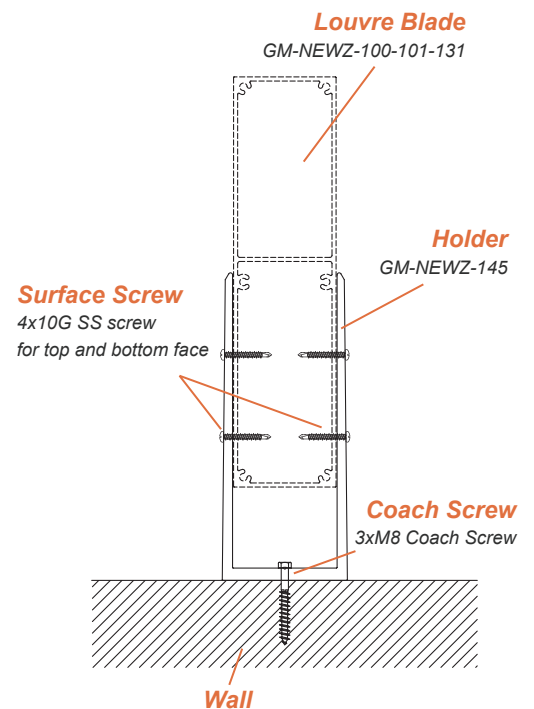
250mm Window Shroud
