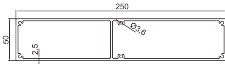
250mm Window Shroud
