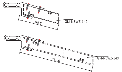
GM-NEWZ-143 160.6x20mm Louvre Blade 2.21kg/m
