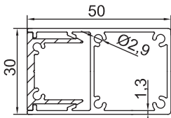
GM-NEWZ-51&53 30x50mm Louvre Blade 1.07kg/m
