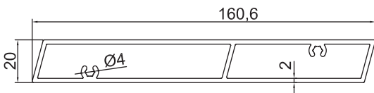
GM-NEWZ-143 160.6x20mm Louvre Blade 2.21kg/m
