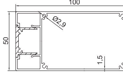
GM-NEWZ-55&53 50x100mm Louvre Blade 1.91kg/m
