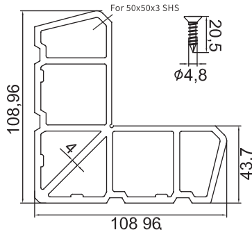
GM-KPM-5511 50x50mm Corner Stake
