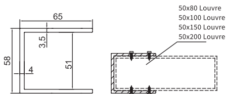
GM-NEWZ-58x65x3.5U 50mm Louvre Blade Holder
