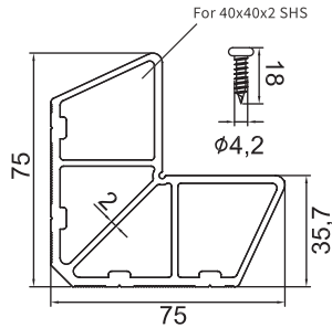
GM-NEWZ-122 40x40mm Corner Stake
