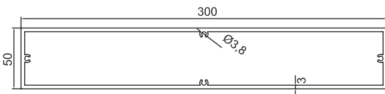
300mm Window Shroud
