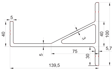
GM-NEWZ-184 Louvre Blade Holder 4.690kg/m
