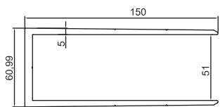
Window Shroud Holder
