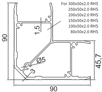
GM-NEWZ-133 50mm Corner Stake
