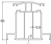
GM-NEWZ-Y13060 A5 Strengthen Frame
