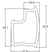
GM-NEWZ-Y13024 Side Frame Extended Ferrule
