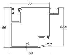
GM-NEWZ-Y13062 A5 Side Frame
