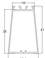
GM-NEWZ-Y13061 A5 Double-Slot Support Bar
