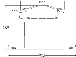
GM-NEWZ-Y13006 Standard Frame
