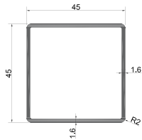
GM-NEWZ-45x45x1.6R 25.6mm Square Hole Weight: 0.783kg/m
