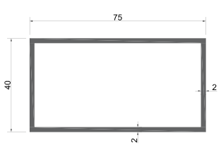
GM-NEWZ-75x40x2 GM-NEWZ-06 Hole Weight: 1.33kg/m
