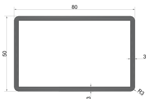
WZ-80x50x3R 25.8mm Square Hole Weight: 2.21kg/m
