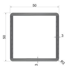
GM-NEWZ-50x50x3R 20mm Square Hole Weight: 1.67kg/m
